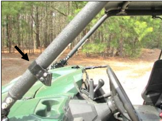
5. Attach the door hinge bracket to the front roll cage bar.
